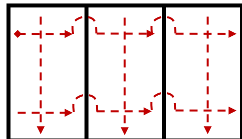
TYPICAL VENTILATION CUT "MULTI-ROLL LOUVER"
